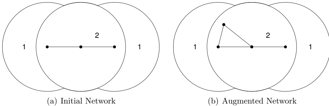
Figure 3-2: Figure (a) illustrates the regions corresponding to the two bi-connected components in the graph. These components share the middle point. Each region is labeled with its rank. Figure (b) illustrates that a point may be selected in the region with the greatest rank that does not bi-connect the network.
