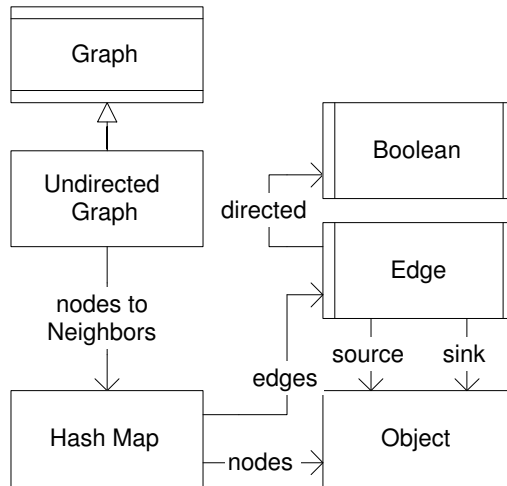
Figure 3-4: The object model for a Graph.
